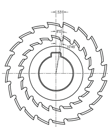
Constant Rake Offset
