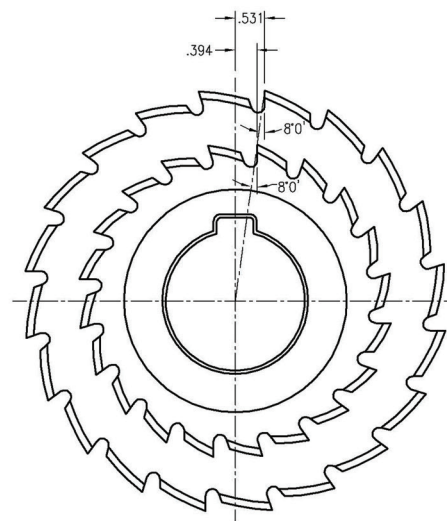
Constant Rake Angle
