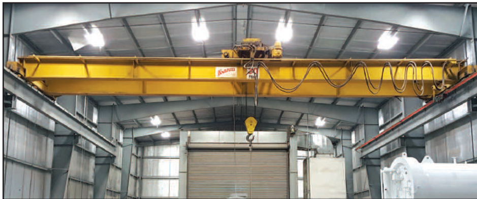
20-Ton x 50' Span Kranco Double Girder Top Running Overhead Bridge Crane
