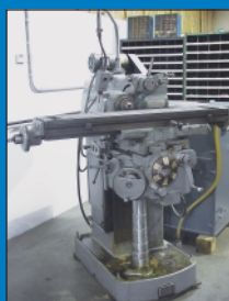
Van Norman Model 24 Universal Horizontal / Vertical Knee Milling Machine
