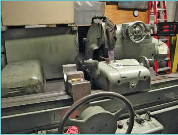
Close-Up View 14" X 168" Landis Wheel Head
