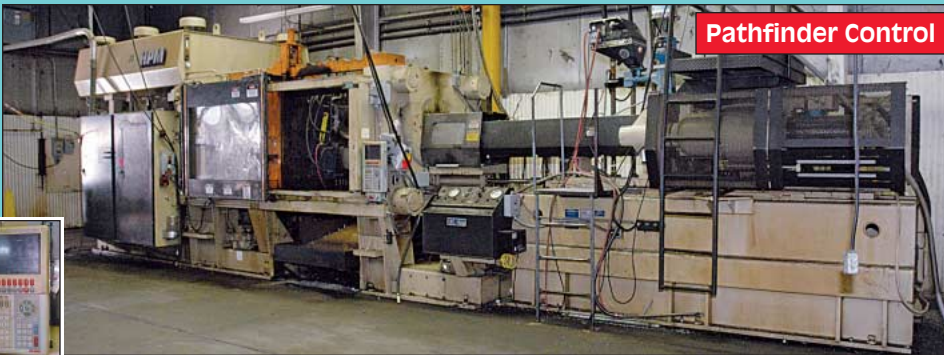
1,000 Ton X 160 Oz. HPM Model 1000-MKII-160 Hydraulic Clamp Injection Molding Machine
