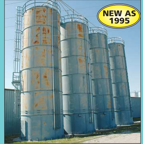
(4) 15' Dia. X 48' High Peabody Tectank Steel Bolt Together Storage Silos
